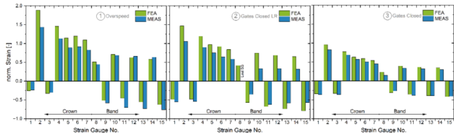
Figure 10. Validation of absolute mean strain extreme conditions.
