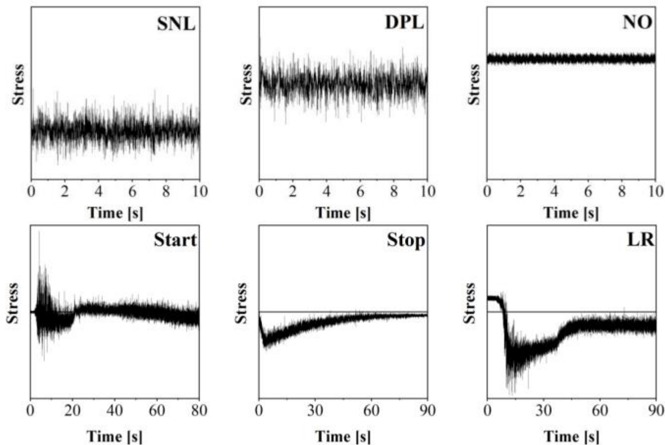
Figure 1. Time Signal for SNL, DPL, NO, Start, Stop and LR
