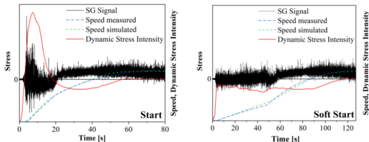
Figure 4. Scaled strain gauge time signal of different Start-ups
