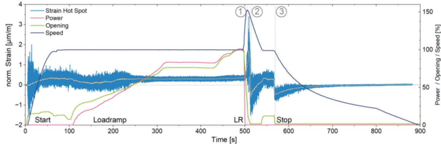
Figure 3. Time signal LR Cycle Band in Hot Spot.
