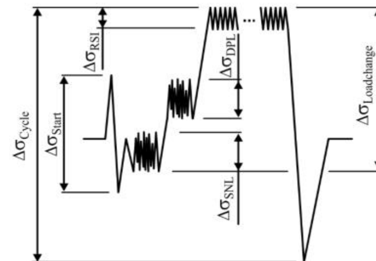
Figure 2. Operation Cycle schematic (based on [3])
