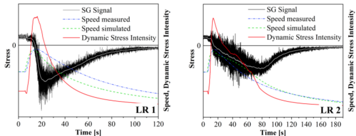
Figure 5. Scaled strain Gauge time signal for two Load Rejections
