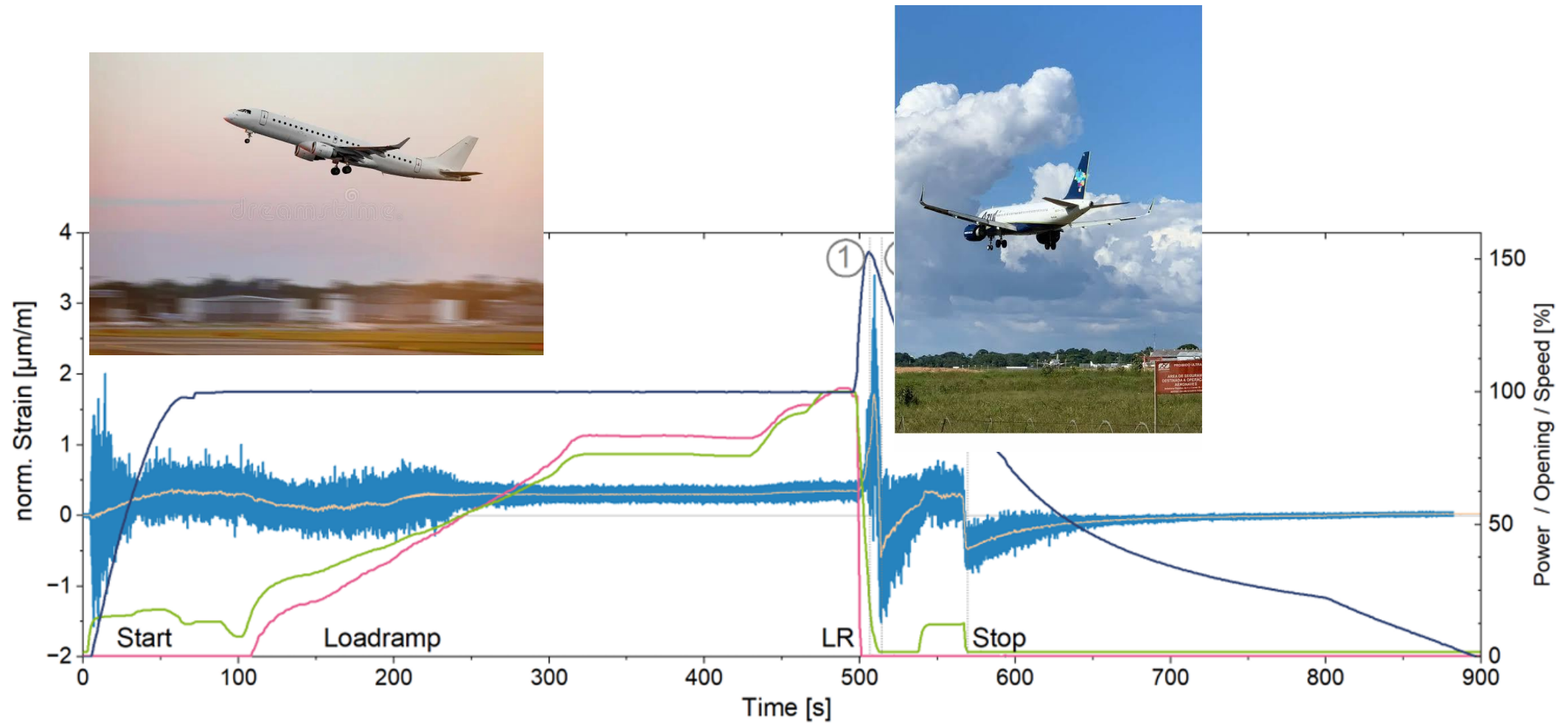
Figure 3. Time signal LR Cycle Band in Hot Spot. [ 2 ]
